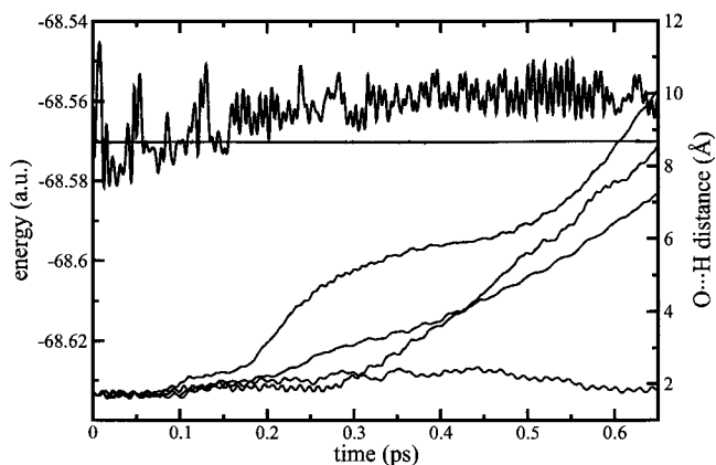
FIG. 4. Total and potential energies (top) as a function of time in a molecular-dynamics simulation of a cyclic tetramer of heavy water in aqueous solution. The total energy contains the contribution of the Nose-Hoover thermostat. The four curves starting at the bottom of the graph represent the evolution of the intermolecular O...H distance between the atoms initially involved in hydrogen bonds.
