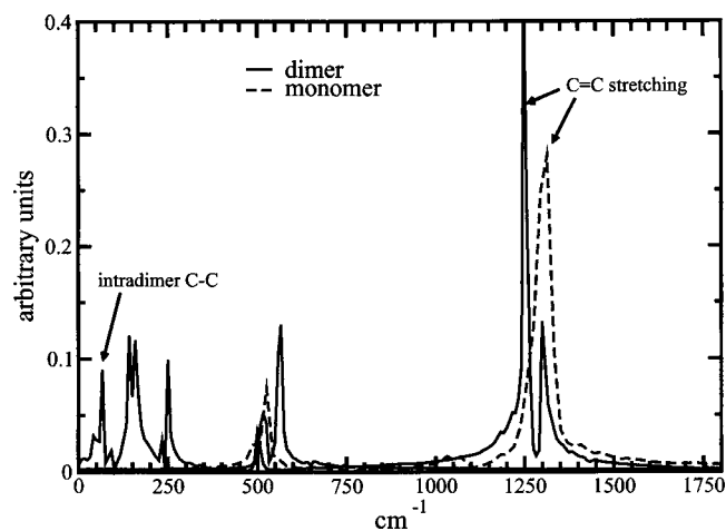
FIG. 8. Characteristic frequencies of the TCNE monomer and dimer extracted from the velocity autocorrelation functions for selected pairs of atoms.
