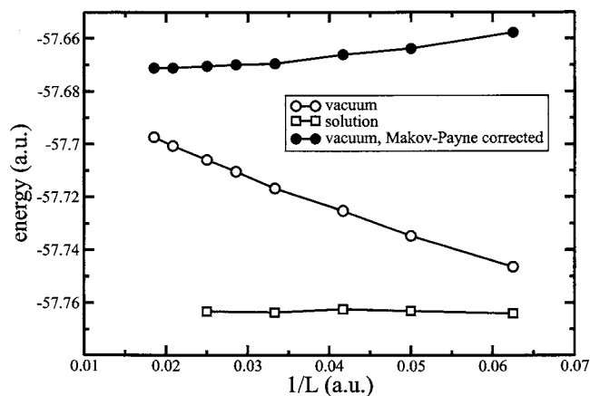
FIG. 2. Total energy of the \text{NO}_3^- anion as a function of the inverse of the lattice parameter, computed in vacuum, in solution, and in vacuum with the Makov-Payne correction up to the leading order.
