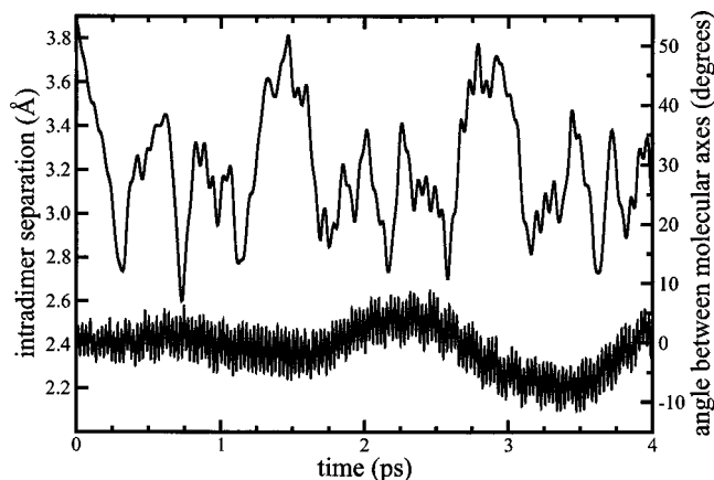
FIG. 7. Time evolution of the intradimer separation (top) and the angle determined by the central \text{C}=\text{C} axes of the two monomers (bottom) during a molecular-dynamics simulation of [\text{TCNE}]_2^{2-} in dichloromethane.
