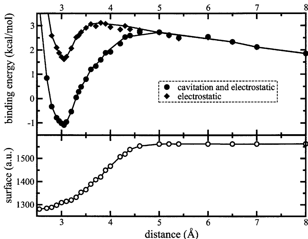
FIG. 6. Upper panel: binding energy of two [\text{TCNE}]^- anions in dichloromethane as a function of its separation, calculated with only the electrostatic contribution to the solvation energy and with both the electrostatic and cavitation contributions. Lower panel: area of the solvation cavity as a function of the separation between the [\text{TCNE}]^- anions. Above 5 Å the cavity splits, and the plotted values correspond to the area of two cavities containing one [\text{TCNE}]^- each.
