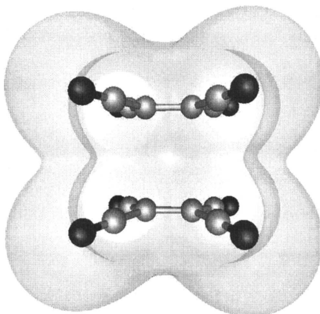
FIG. 5. Optimized structure of a dimer of [TCNE]^- in dichloromethane, enclosed by an electronic density isosurface at 0.00078e delimiting the solvation cavity. Carbon atoms in light gray and nitrogen atoms in dark.
