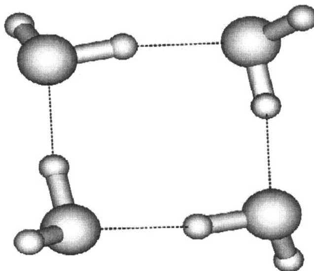
FIG. 3. Cluster of \text{D}_2\text{O} molecules used as starting configuration in the molecular-dynamics simulations which results are reported in Fig. 4.
