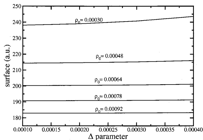
FIG. 1. Cavity area of a water molecule as a function of \Delta (thickness parameter used to evaluate the area, see text) for several values of the electronic density threshold \rho_0 .
