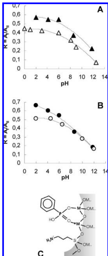
Figure 8. Evolution of the R = A_1/A_{11} XPS peak intensity ratio with pH for Z82 (A) and T82 (B). Films were analyzed after template extraction (open symbols) or after exposing to PP solutions (closed symbols). Continuous curves are a guide to the eye. (C) Scheme of the ammonium conformation on the PP-modified pore surface.
